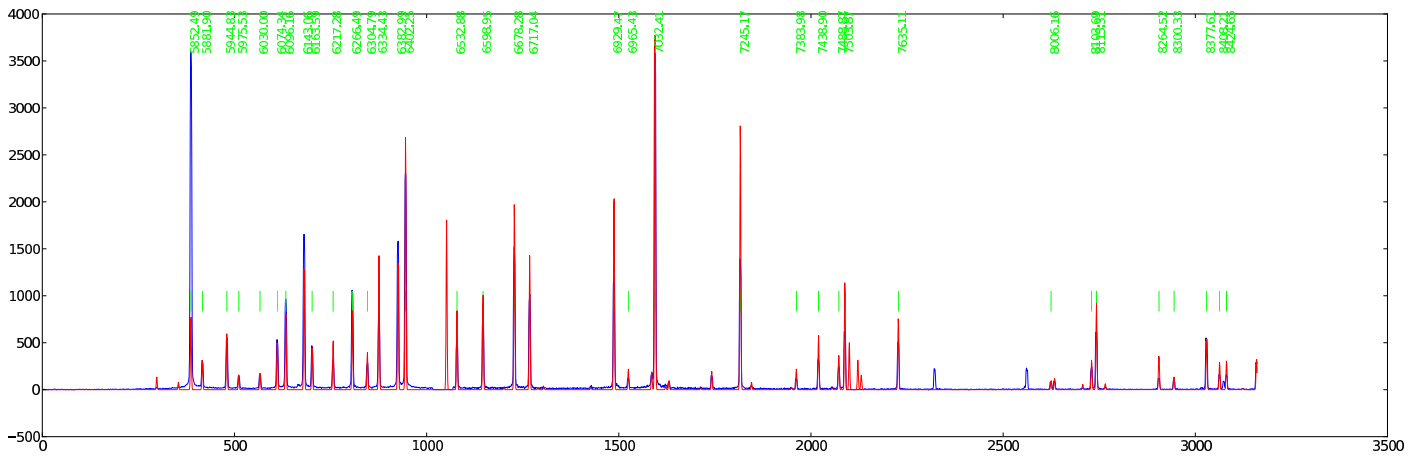
Figure 22: 0122 — 075: Ne PG0900 GR = 18.500 AR = 37.007 \lambda\lambda = 5473 - 8491
