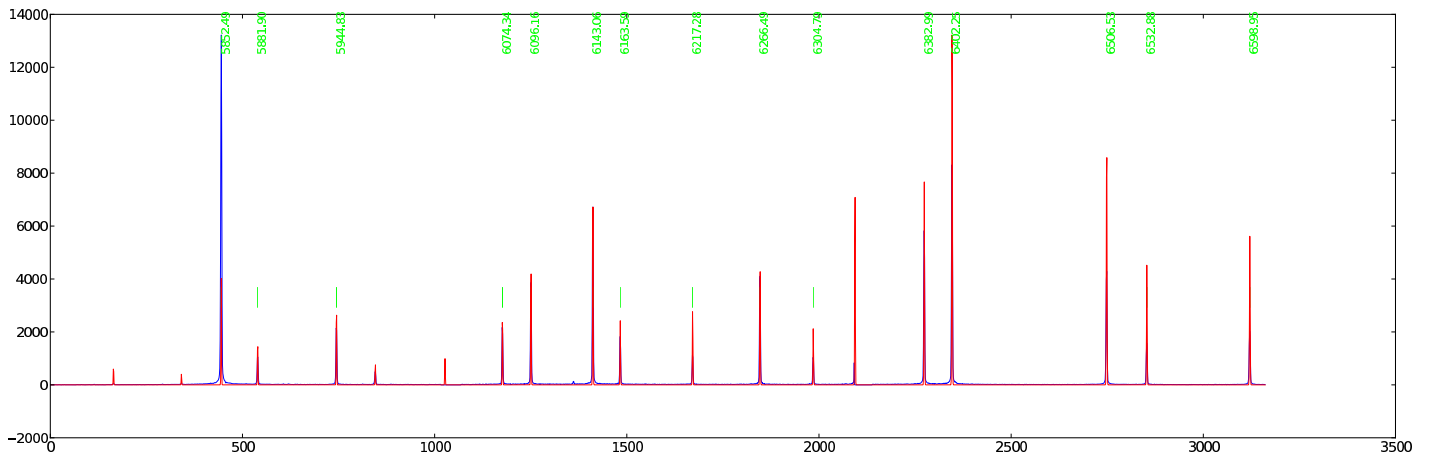
Figure 2: 0909 — 005: Ne PG2300 GR = 45.502 AR = 91.011 \lambda\lambda = 5714 - 6607
