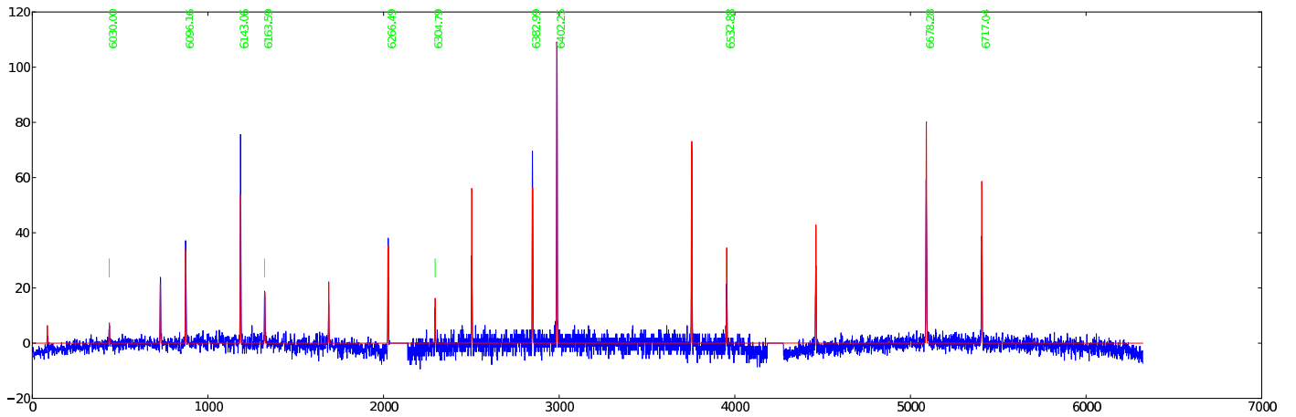
Figure 4: 0908 — 005: Ne PG2300 GR = 47.748 AR = 95.512 \lambda\lambda = 5962 - 6823
