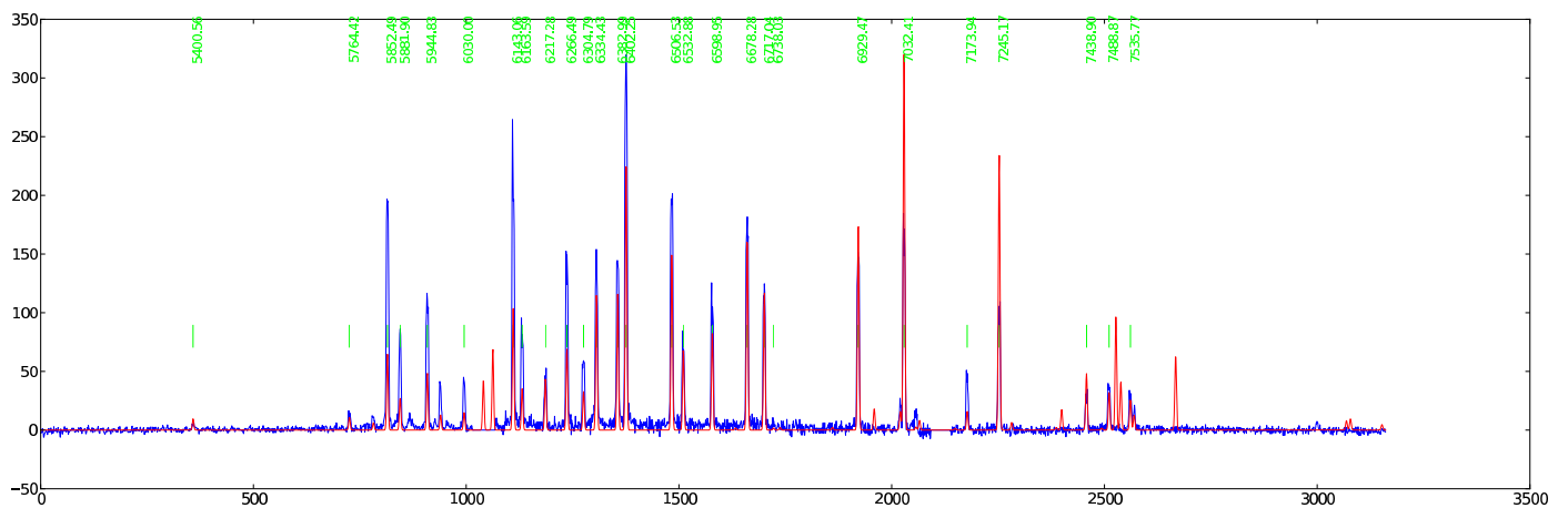
Figure 21: 1229 — 050: Ne PG0900 GR = 17.378 AR = 34.753 \lambda\lambda = 5054 - 8090
