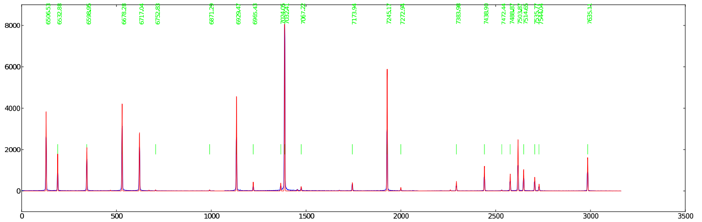
Figure 9: 0114 — 045: Ne PG1800 GR = 45.550 AR = 98.524 \lambda\lambda = 7860 - 8849
