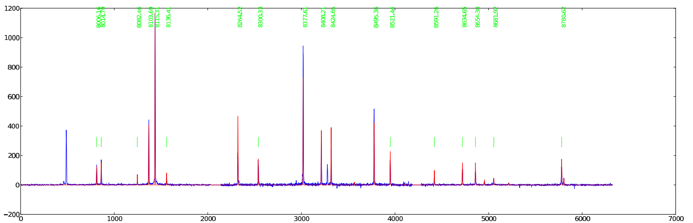
Figure 9: 0114 — 045: Ne PG1800 GR = 45.550 AR = 98.524 \lambda\lambda = 7860 - 8849
