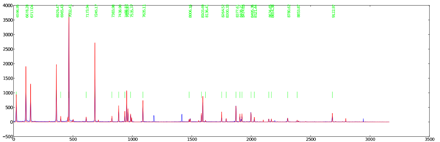
Figure 24: 1123 — 143: Ne PG0900 GR = 21.503 AR = 43.000 \lambda\lambda = 6575 - 9545
