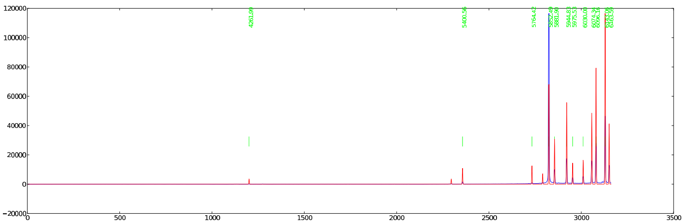
Figure 15: 1123 — 139: Ne PG0900 GR = 12.127 AR = 24.252 \lambda\lambda = 3072 - 6172
