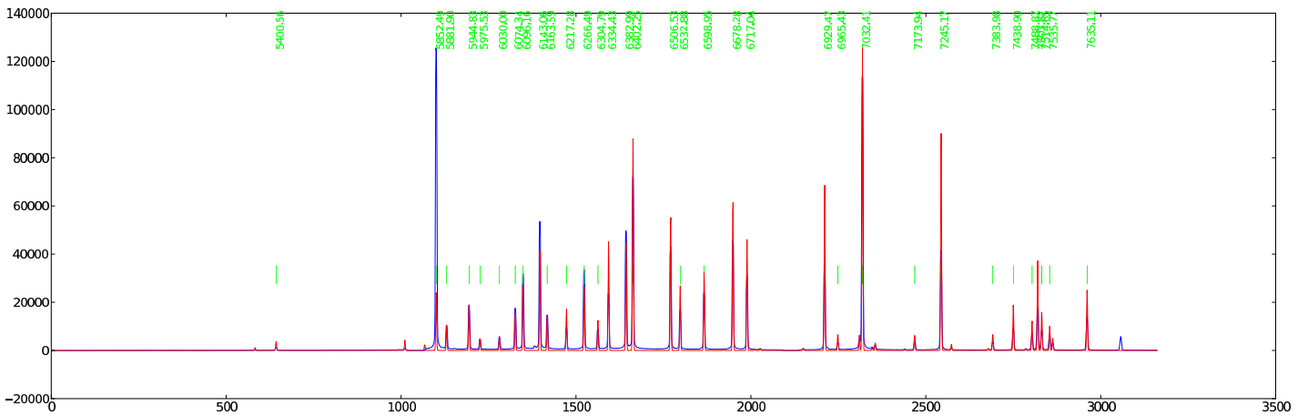
Figure 19: 1123 — 141: Ne PG0900 GR = 16.625 AR = 33.251 \lambda\lambda = 4763 - 7816
