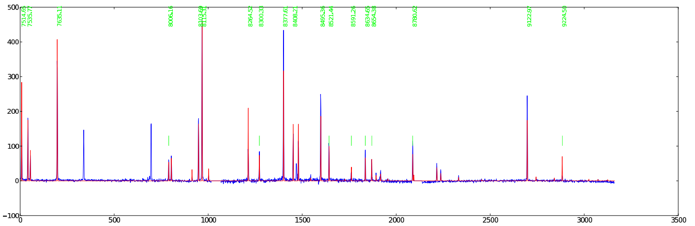
Figure 14: 0224 — 044: Ne PG1300 GR = 33.502 AR = 67.005 \lambda\lambda = 7512 - 9373
