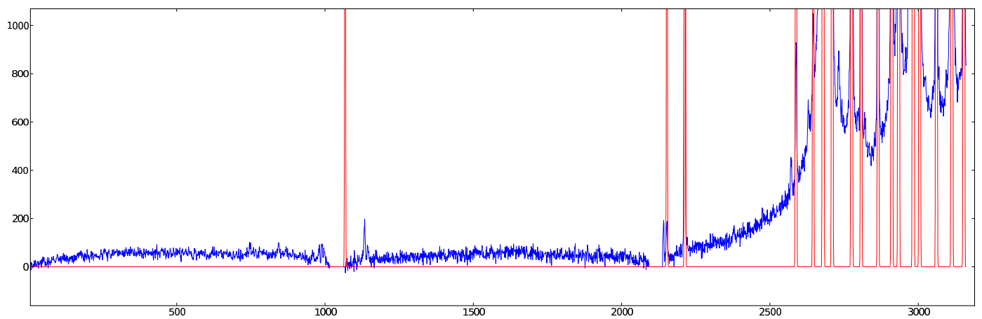
Figure 18: 1123 — 140 (zoom): Ne PG0900 GR = 12.502 AR = 25.002 \lambda\lambda = 3177 - 6311
