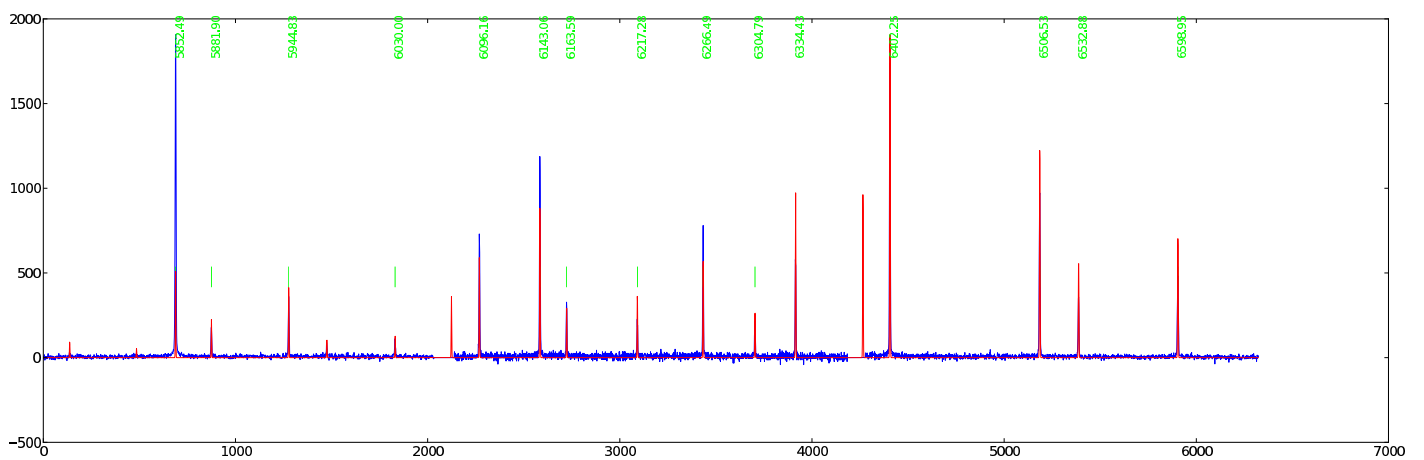
Figure 3: 0911 — 061: Ne PG2300 GR = 47.000 AR = 91.760 \lambda\lambda = 5743 - 6650
