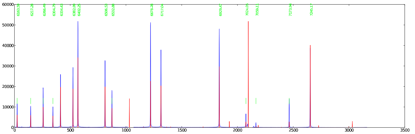
Figure 7: 1224 — 008: Ne PG1800 GR = 38.000 AR = 76.016 \lambda\lambda = 6152 - 7430
