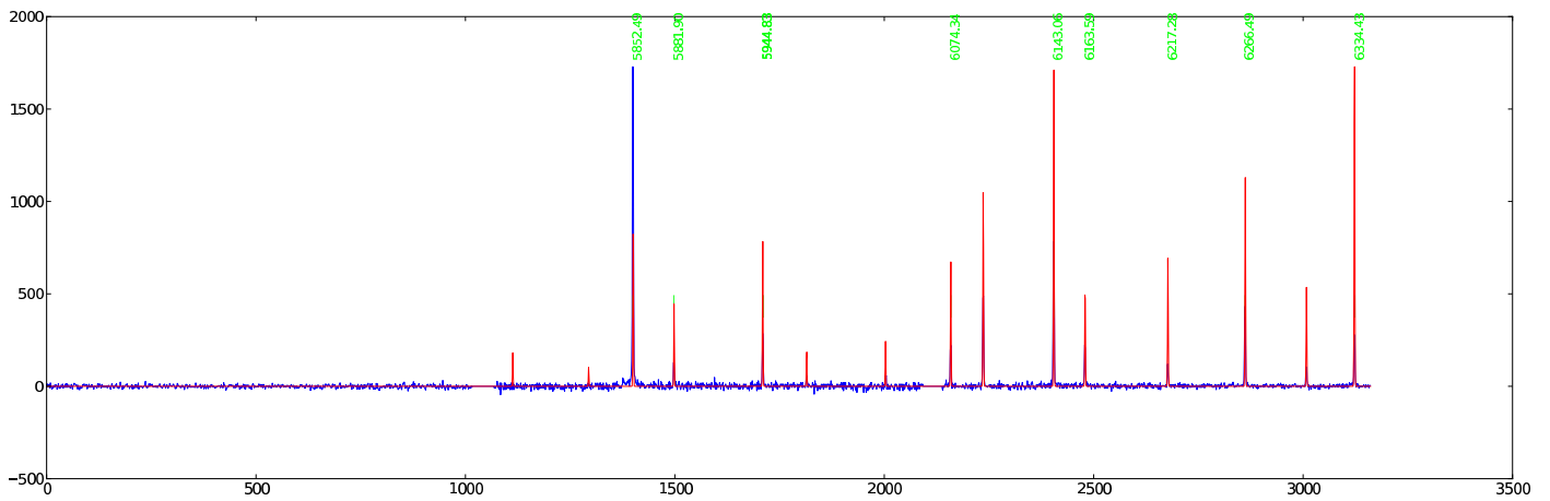
Figure 1: 0926 — 042: Ne PG2300 GR = 42.875 AR = 85.762 \lambda\lambda = 5490 - 6314
