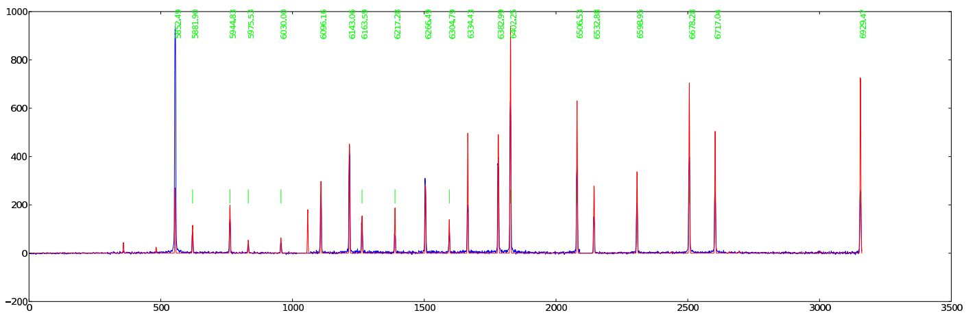
Figure 6: 0318 — 002: Ne PG1800 GR = 34.625 AR = 69.258 \lambda\lambda = 5602 - 6931
