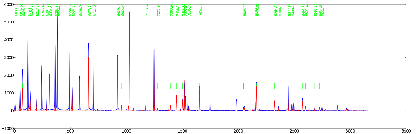
Figure 23: 1006 — 104: Ne PG0900 GR = 20.003 AR = 40.003 \lambda\lambda = 6029 - 9026
