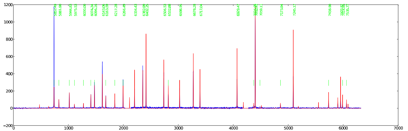
Figure 12: 0320 — 034: Ne PG1300 GR = 28.250 AR = 56.517 \lambda\lambda = 6259 - 8218
