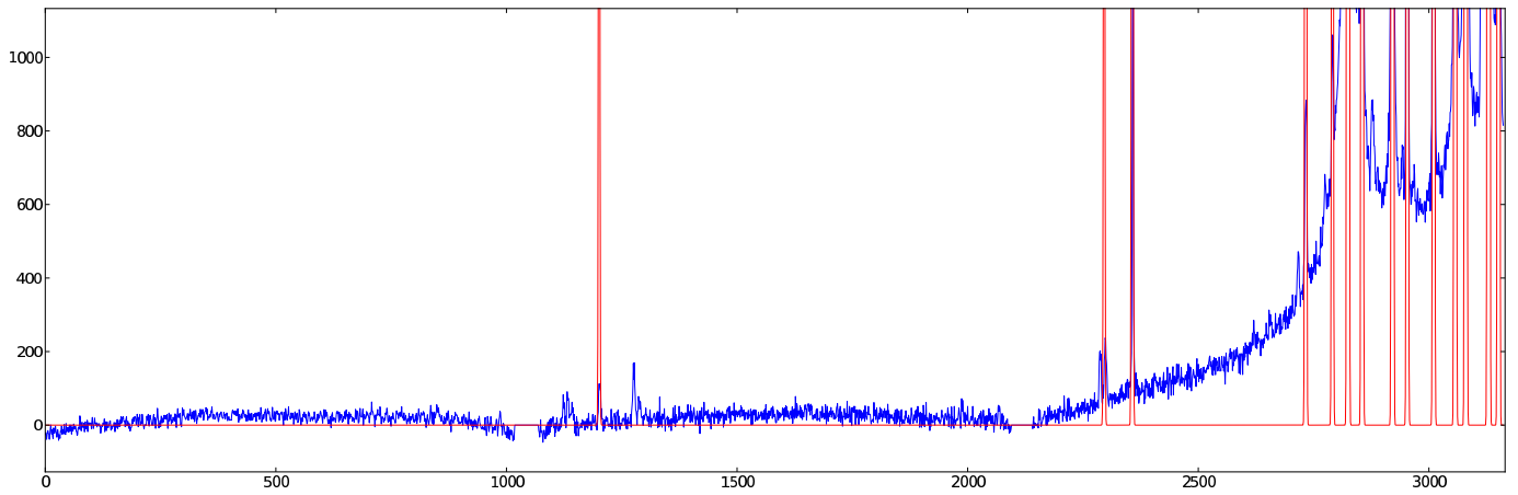
Figure 17: 1123 — 140: Ne PG0900 GR = 12.502 AR = 25.002 \lambda\lambda = 3177 - 6311
