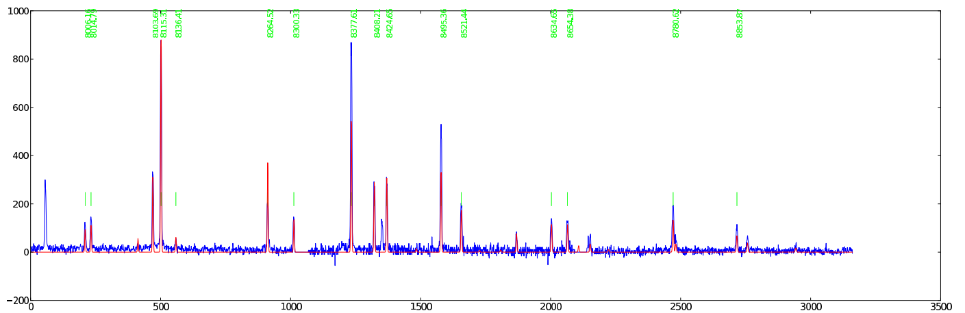
Figure 10: 1111 — 103: Ne PG1800 GR = 50.000 AR = 100.009 \lambda\lambda = 7928 - 8979
