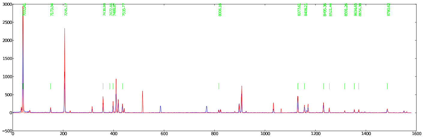
Figure 13: 0319 — 026: Ne PG1300 GR = 31.250 AR = 62.503 \lambda\lambda = 6981 - 8882
