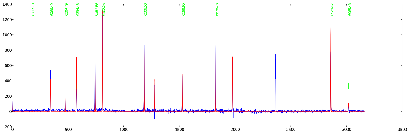
Figure 5: 1114 — 105: Ne PG2300 GR = 49.627 AR = 99.258 \lambda\lambda = 6164 - 6996
