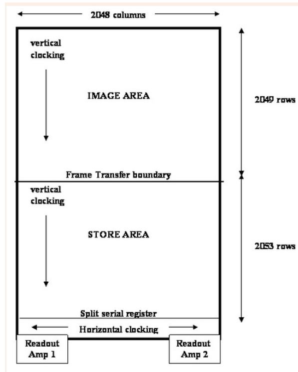
Figure A3. SALTICAM schematic for one of the two CCDs.
