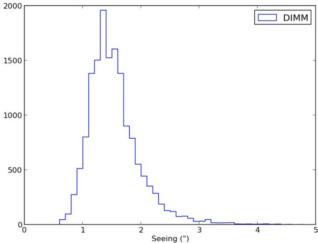
Figure 6 - Seeing histogram from our DIMM for the 2013-1 semester (1 May 2013 - 31 October 2013). The y-axis indicates the number of hours at that given seeing.
