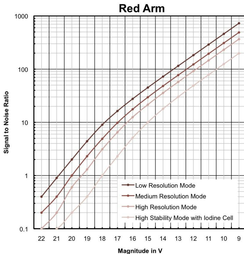
Figure 11. The expected signal to noise ratio (S/N) of SALT HRS as a function of stellar visual
