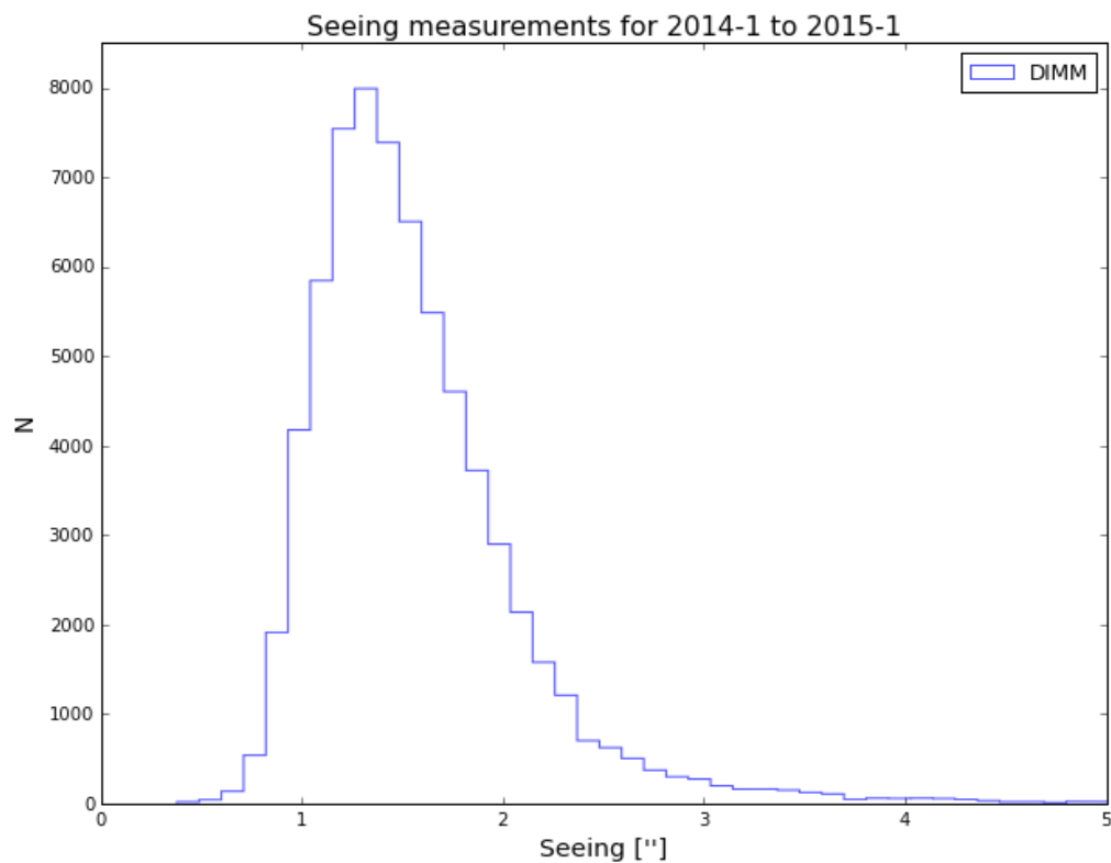
Figure 6 - Seeing histogram from the SAAO DIMM for the period 2014-1 to 2015-1 (1 May 2014 - 31 October 2015). The y-axis indicates the number of seeing measurements at that given seeing.
