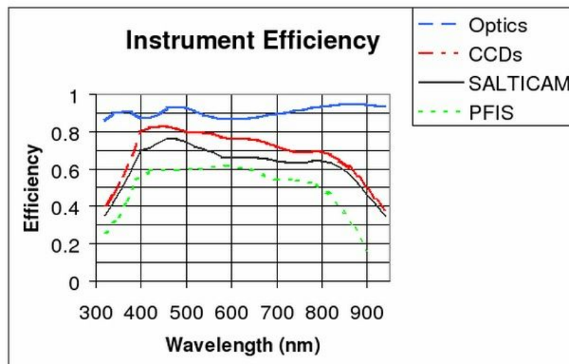
Figure 1. Instrument Efficiencies
