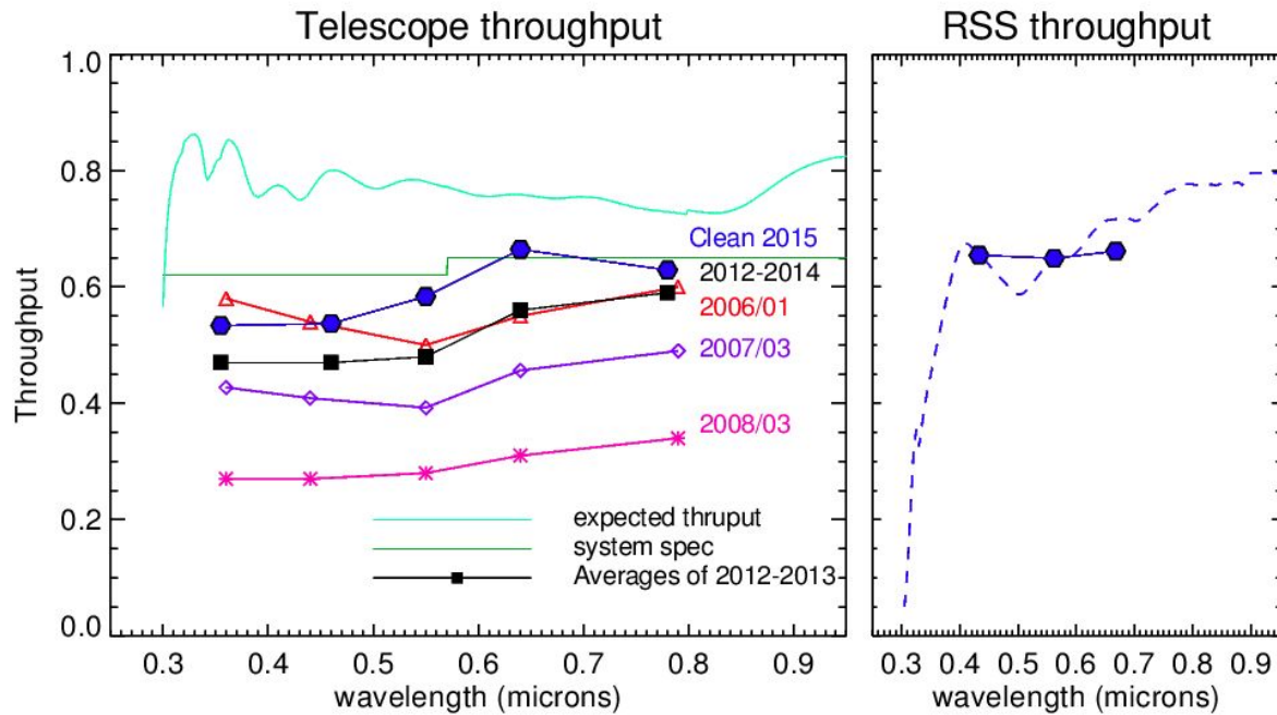
Figure 8. Current and historical telescope throughput values are shown at left compared to expectations. The most recent values after the ADC was cleaned are shown in dark blue. Measurements correspond to 7-10 best quality segments, so the implemented values in the Simulator are 15-20% worse to describe a typical track. The right panel shows, as the dashed line, the RSS optics throughput as derived by Ken Nordsieck in 2013 adjusted by the factor of approximately 1.6 improvement in efficiency after the 2014 RSS intervention and 2015 ADC clean. The blue points show measured values from on-sky photometry in June 2015. All these values are incorporated in the current instrument Simulator tools and are kept up-to-date.
