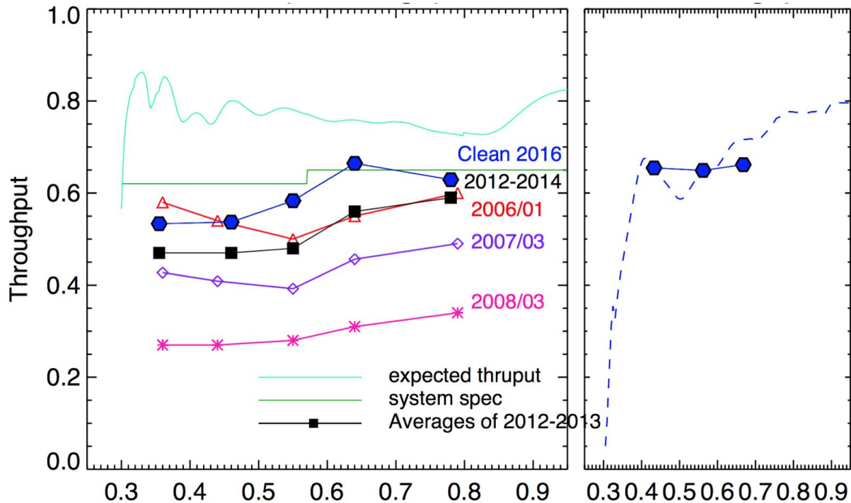
Figure 4.2: Left: Current and historical telescope (that is, SALTICAM) throughput values for different wavelengths (in micrometer) are compared to expectations. The most recent values are shown in dark blue. Measurements correspond to the 7–10 best quality mirror segments. Right: RSS optics throughput values. The dashed line was derived by Ken Nordsieck in 2013 and has been adjusted by the factor of approximately 1.6 improvement in efficiency due to the 2014 RSS intervention and 2015 ADC clean. The blue points show mean values from measured on-sky photometry in 2015, 2016, and 2017, when they have stayed quite stable.
