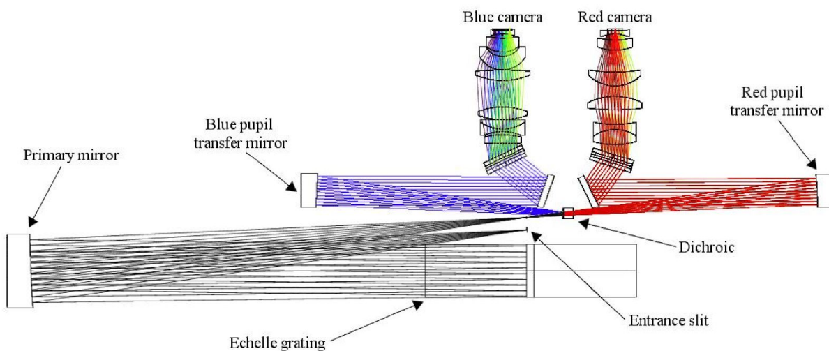
Figure A.21: Optical path for the HRS.
