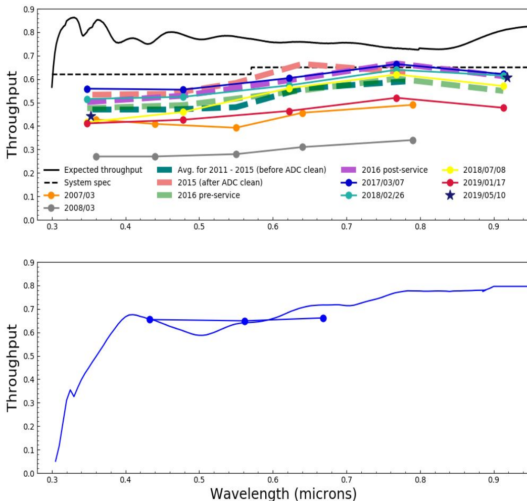
Figure 4.2: Top: Current and historical telescope (that is, SALTICAM) throughput values for different wavelengths (in micrometer) are compared to expectations. The most recent values are indicated with the dark blue stars (only the first and last filters are shown here because the exposure times were long enough to eliminate the shutter effect of SALTICAM, while those in the middle were not). Measurements correspond to the 7–10 best quality mirror segments. Bottom: RSS optics throughput values. The line was derived by Ken Nordsieck in 2013 and has been adjusted by a factor of approximately 1.6 improvement in efficiency due to the 2014 RSS intervention and 2015 ADC clean. The blue points show mean values from
