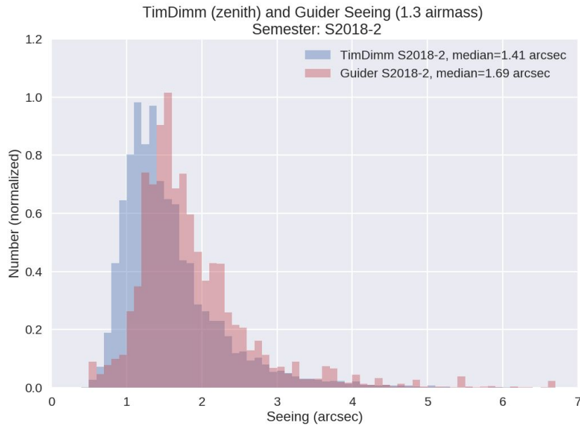
Figure 3.1: Seeing histograms from the SAAO DIMM and the SALT guider. The data are taken from the same period of time in 2018. Note that the guider data are not corrected for the average airmass of SALT observations during this period, so the guider data are actually better than the DIMM (which is closer to the ground). The PIs select their seeing restriction based on the intrinsic Zenith value and they now should expect a similar image quality delivered on the detector.
