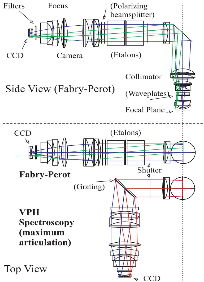
Figure A.19: RSS optical path with Fabry-Pérot
