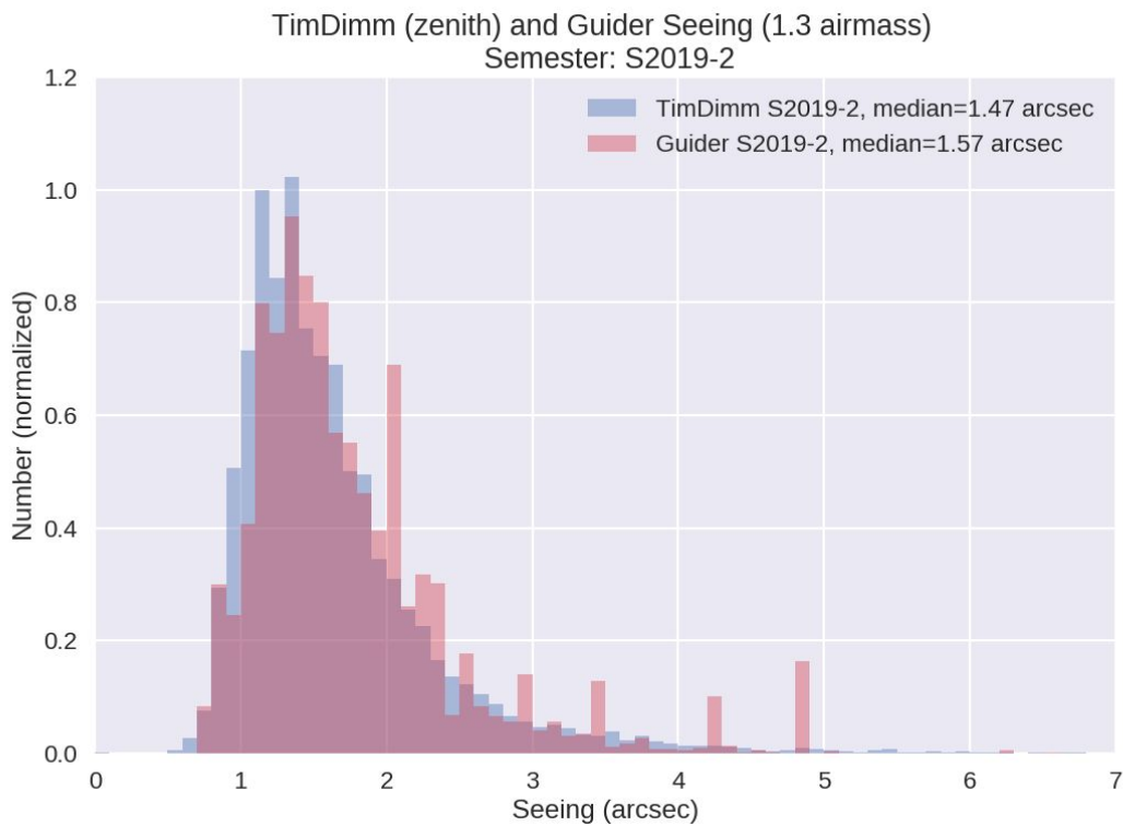
Figure 3.1: Seeing histograms from the SAAO DIMM and the SALT guider. The data are taken from the same period of time in 2019 and 2020. Note that the guider data are not corrected for the average airmass of SALT observations during this period, so the guider data are actually better than the DIMM (which is closer to the ground). The PIs select their seeing restriction based on the intrinsic Zenith value and they now should expect a similar image quality delivered on the detector.
