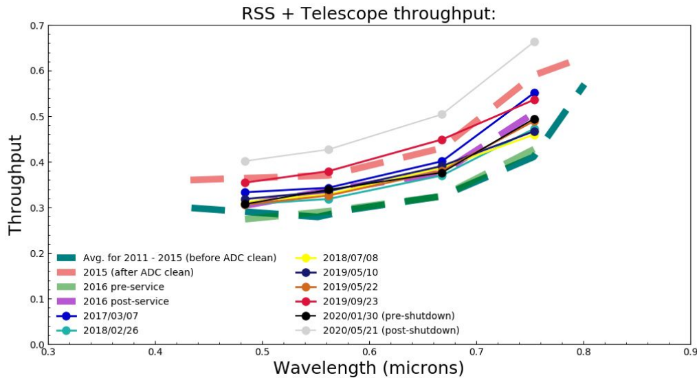
Figure 4.3: Current and historical RSS + telescope throughput values for different wavelengths (in micrometers). The most recent values are indicated with the light grey circles.
