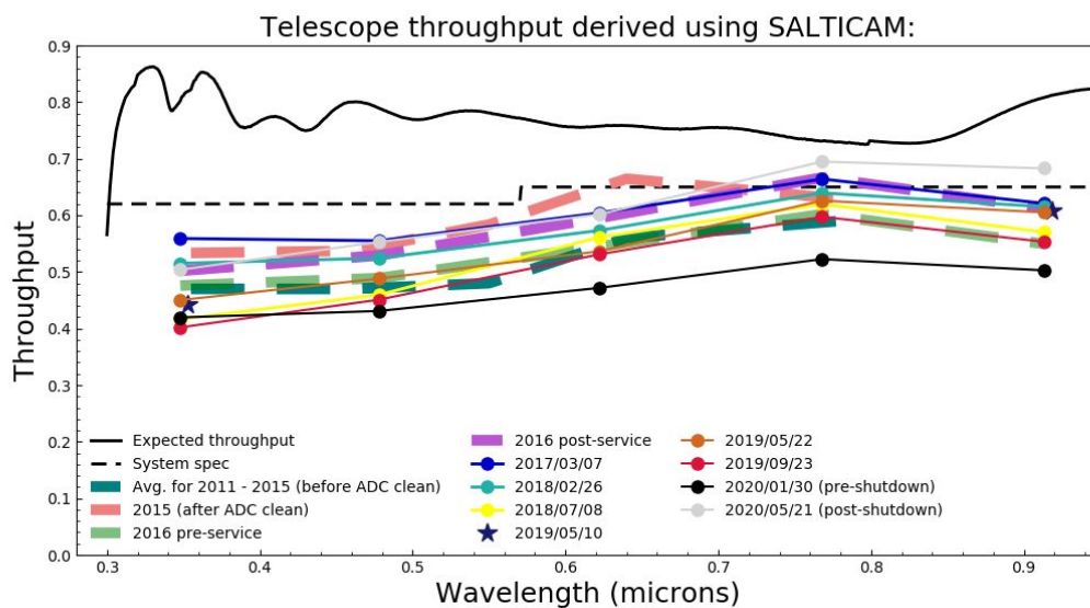
Figure 4.2: Current and historical telescope (that is, SALTICAM) throughput values for different wavelengths (in micrometers) are compared to expectations. The most recent values are indicated with the light grey circles. Measurements correspond to the 7–10 best quality mirror segments.
