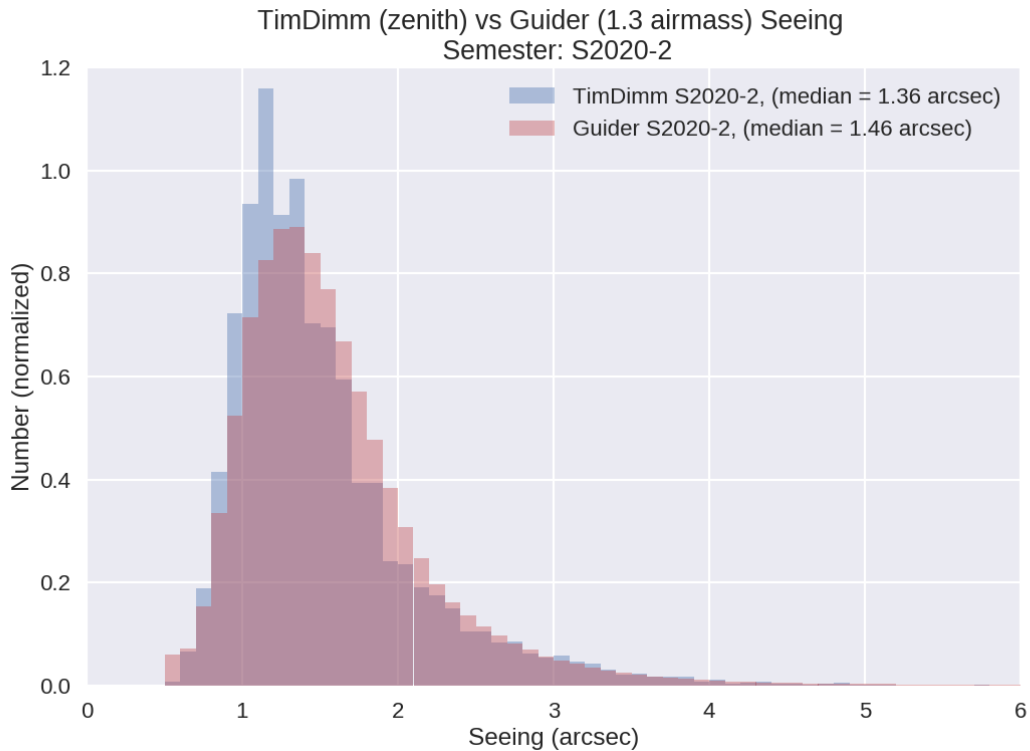
Figure 3.1: Seeing histograms from the SAAO DIMM and the SALT guider. The data are taken from the same period of time in 2020 and 2021. Note that the guider data are not corrected for the average airmass of SALT observations during this period, so the guider data are actually better than the DIMM (which is closer to the ground). The PIs select their seeing restriction based on the intrinsic Zenith value and they now should expect a similar image quality delivered on the detector.
