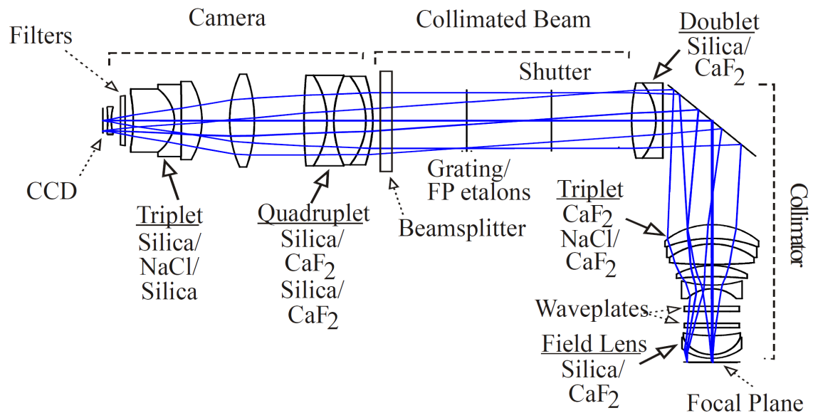
Figure A.14: Top: technical diagram of RSS; bottom: RSS optical path.
