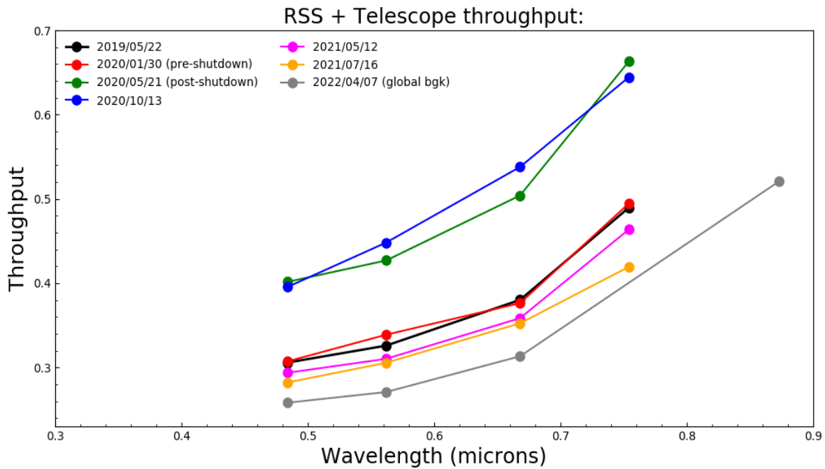
Figure 4.3: Current and historical RSS + telescope throughput values for different wavelengths (in micrometres). The most recent values are indicated with the grey circles.
