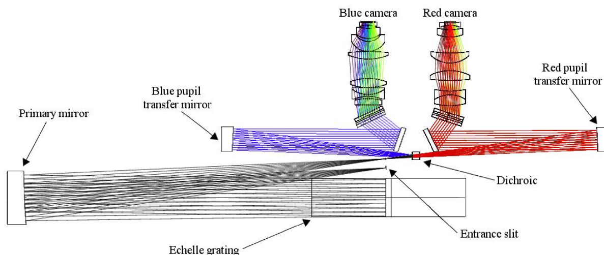
Figure A.21: Optical path for the HRS.
