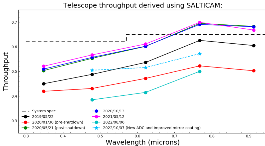
Figure 4.2: Current and historical telescope (that is, SALTICAM) throughput values for different wavelengths (in micrometres) are compared to expectations. The most recent values are indicated with the cyan stars. Measurements correspond to the 7–10 best quality mirror segments.
