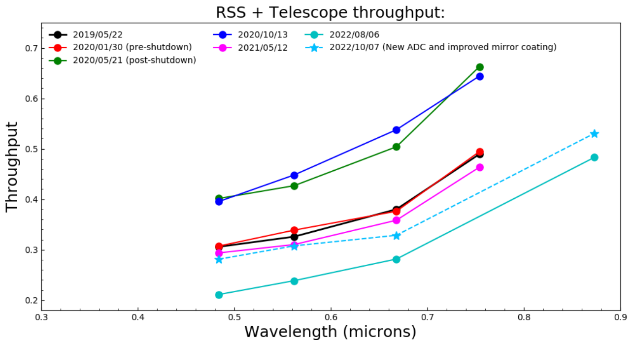
Figure 4.3: Current and historical RSS + telescope throughput values for different wavelengths (in micrometres). The most recent values are indicated with the cyan stars.
