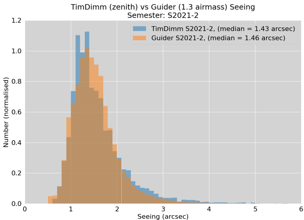
Figure 3.1: Seeing histograms from the SAAO DIMM and the SALT guider. The data are taken from the same period of time in 2021. Note that the guider data are not corrected for the average airmass of SALT observations during this period, so the guider data are actually better than the DIMM (which is closer to the ground). The PIs select their seeing restriction based on the intrinsic Zenith value and they now should expect a similar image quality delivered on the detector.
