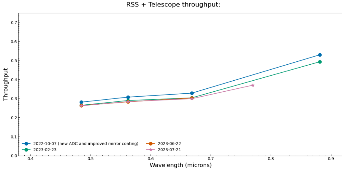
Figure 4.3: Current and historical RSS + telescope throughput values for different wavelengths (in micrometres). The most recent values are indicated with the pink stars.
