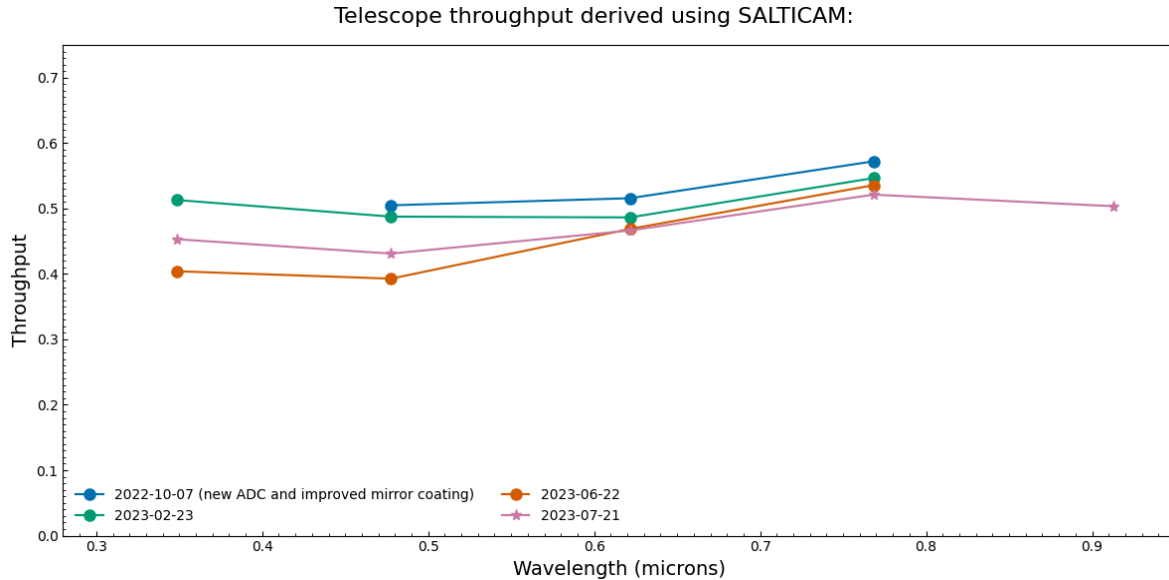
Figure 4.2: Current and historical telescope (that is, SALTICAM) throughput values for different wavelengths (in micrometres). The most recent values are indicated with the pink stars. Measurements correspond to the 7–10 best quality mirror segments.
