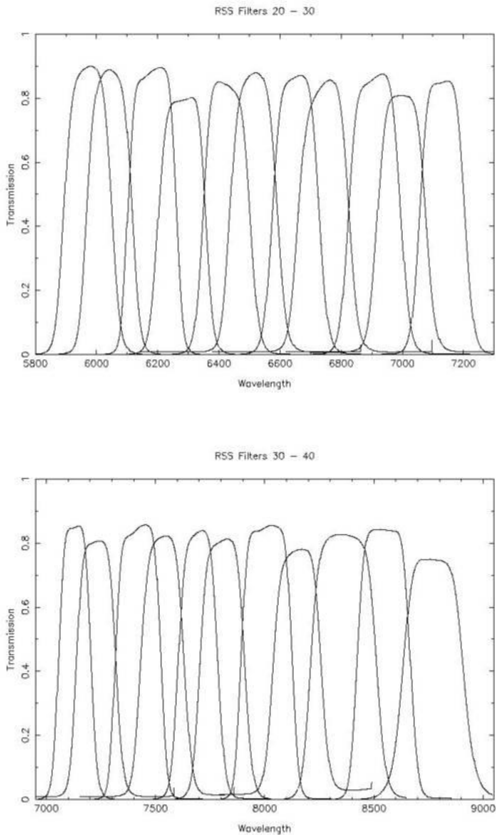
Figure A.19: Filter transmission curves for the FP narrow-band filters.
