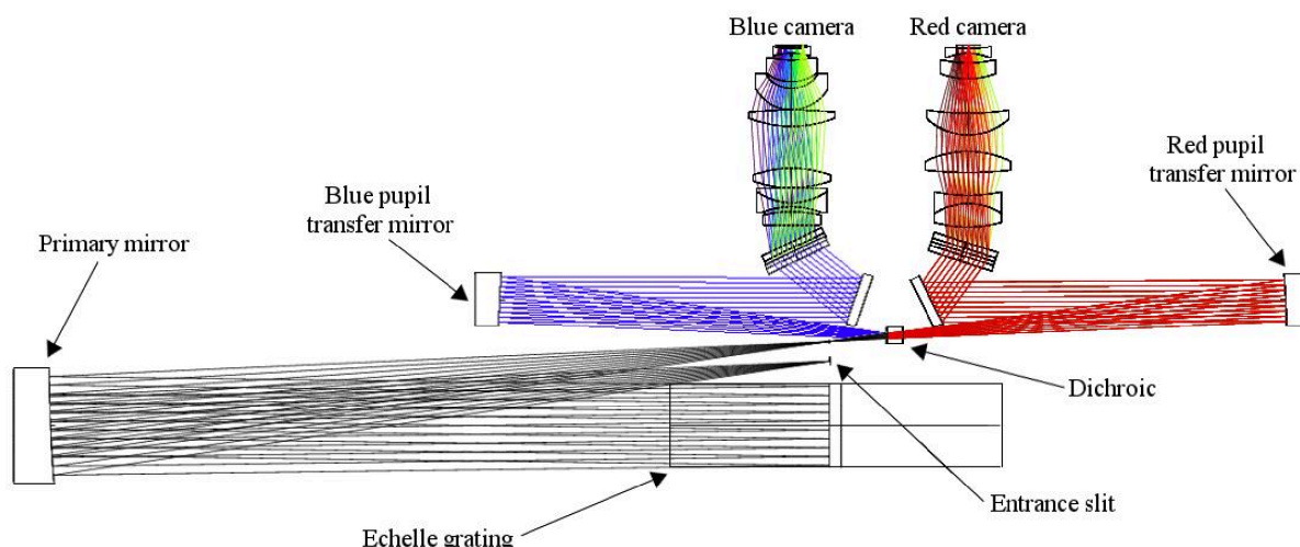
Figure A.20: Optical path for the HRS.
