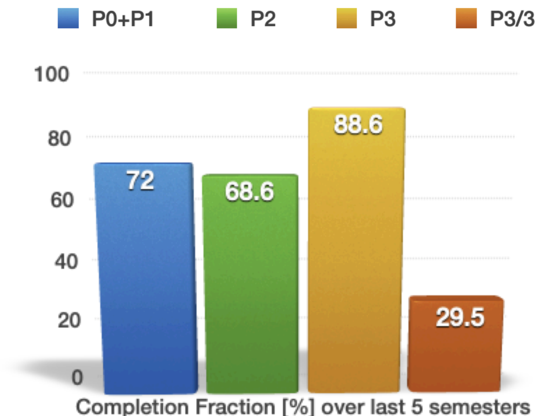
Figure 1.2: Completeness of Observing Blocks by priority, for 2021-2 to 2023-2. The P3 completion is divided by 3, as it's over-subscribed by a factor of 3.
