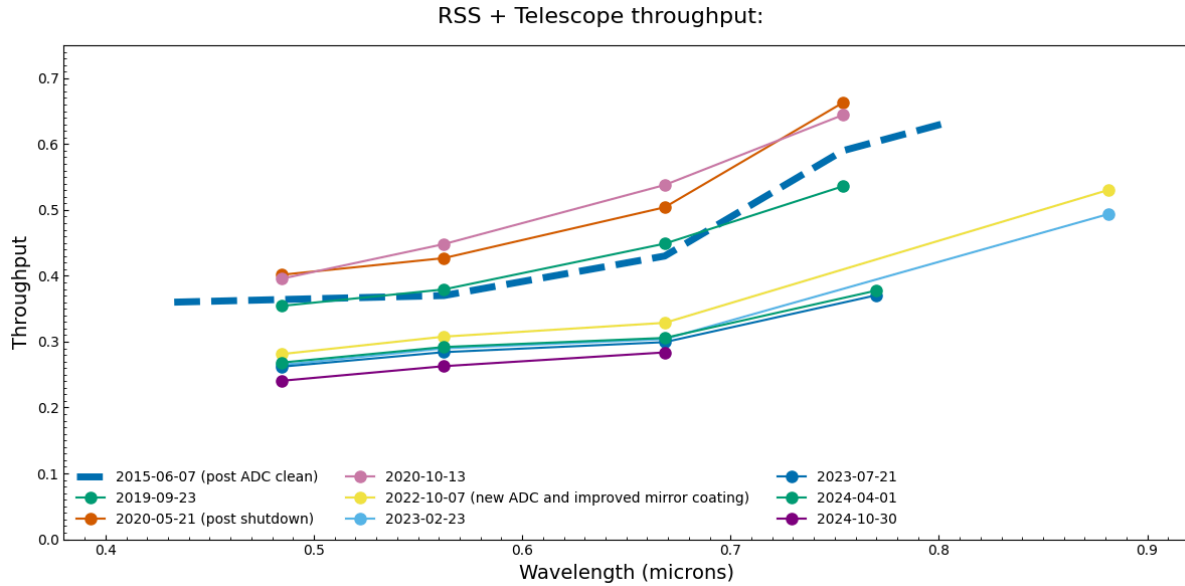
Figure 4.3: Current and historical RSS + telescope throughput values for different wavelengths (in micrometres). The most recent values are indicated with the purple points.
