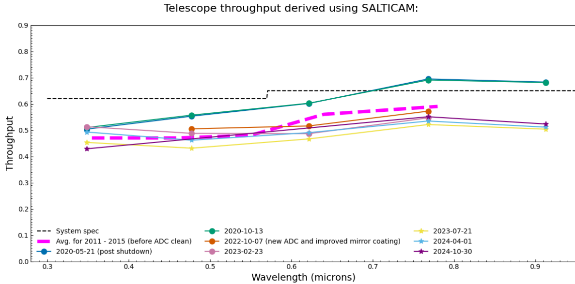
Figure 4.2: Current and historical telescope (that is, SALTICAM) throughput values for different wavelengths (in micrometres). The most recent values are indicated with the purple stars. Measurements correspond to the 7–10 best quality mirror segments.
