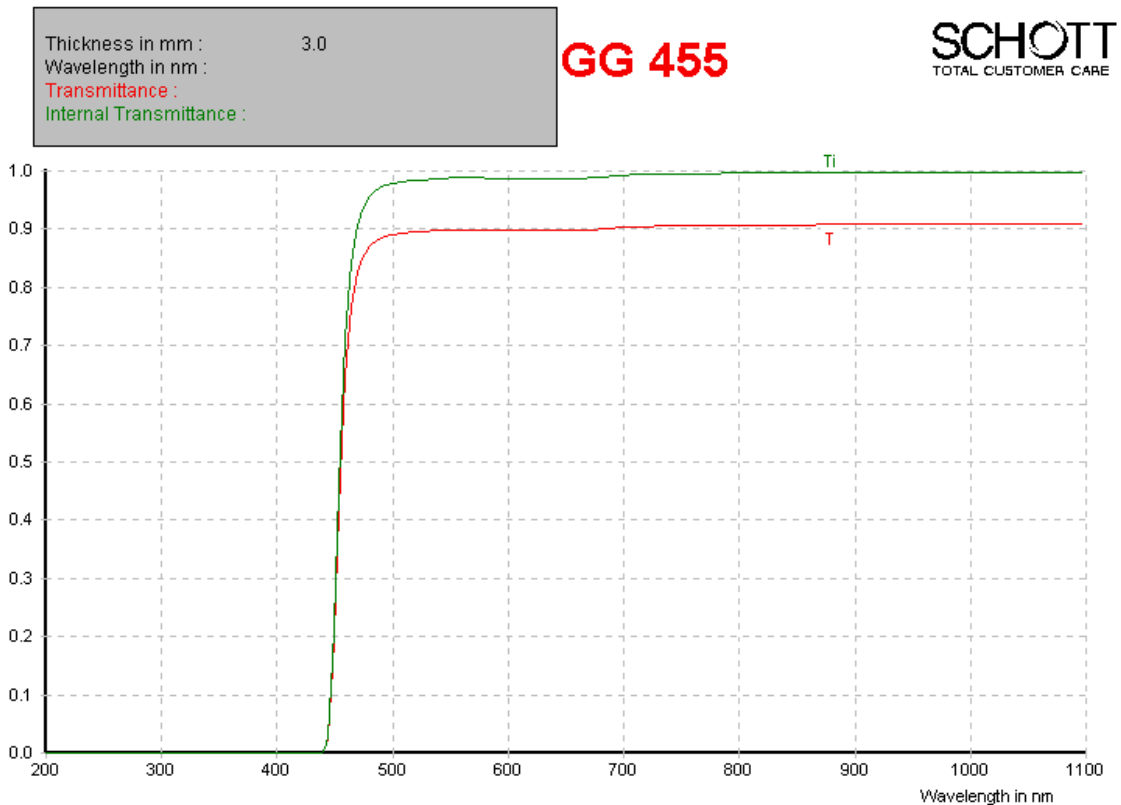
Figure A.18: Transmission curve for Blue filter PC04600.
