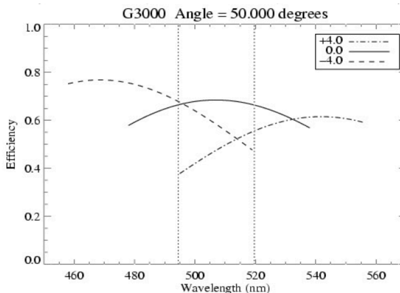
Figure 7.3: Example of the effect of blaze-angle on wavelength range and efficiency in MOS mode. Shown are the default case (on-axis) and the two extreme cases of having an object at
