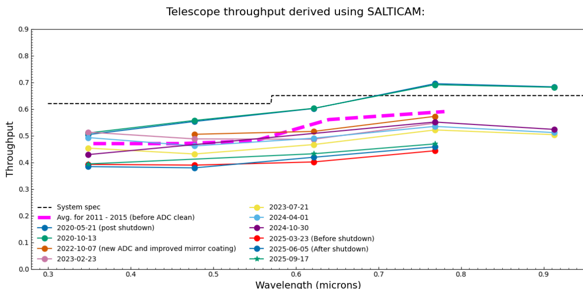
Figure 4.2: Current and historical telescope (that is, SALTICAM) throughput values for different wavelengths (in micrometres). The most recent values are indicated with the green
