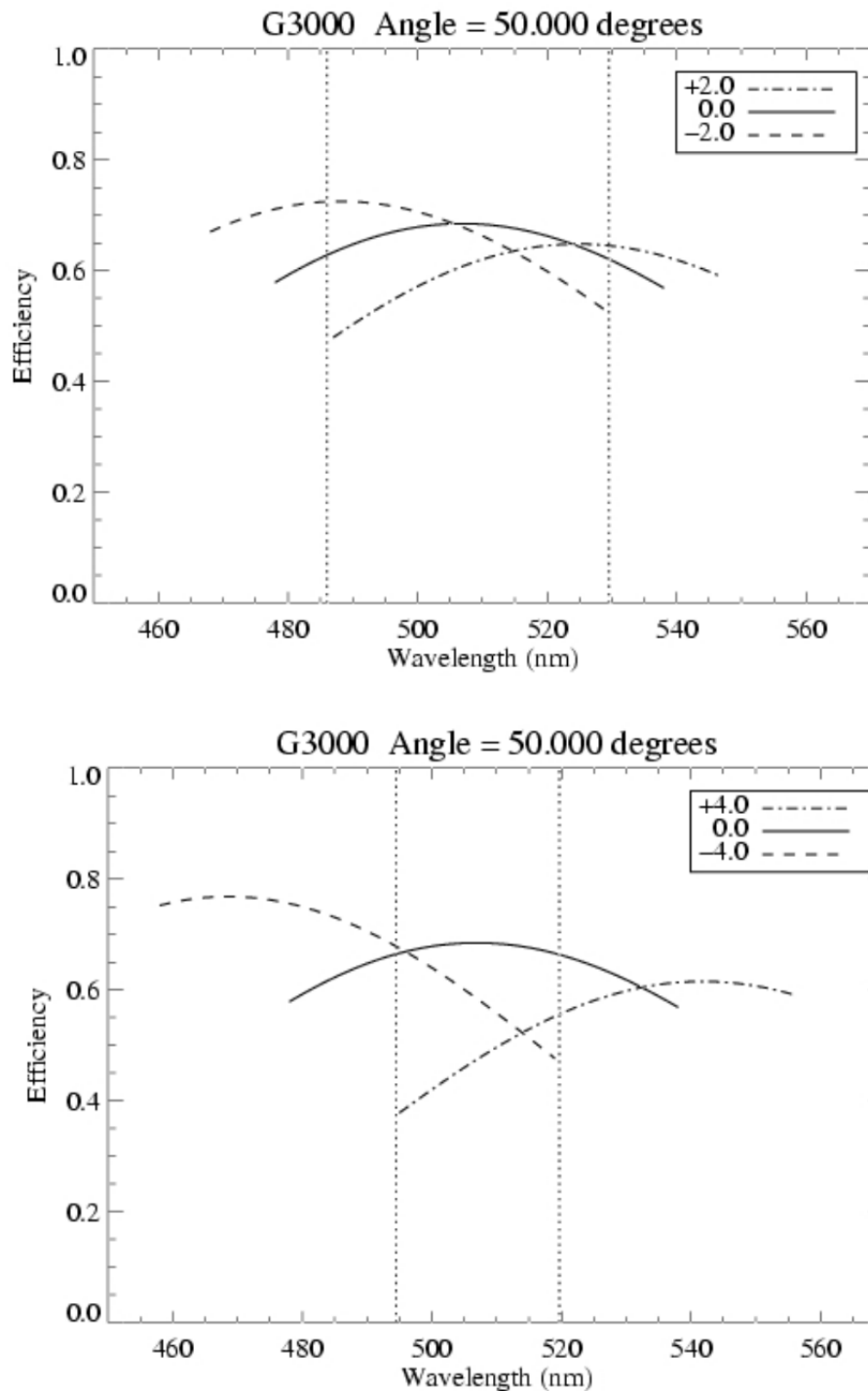
Figure A.19: Wavelength coverage and efficiency for the on-axis and two off-axis positions at \pm 2' (top panel) and \pm 4' (bottom panel).
