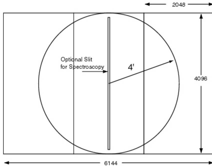
Figure A.15: Old RSS detector system with slit position.
