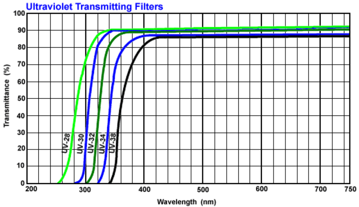
Figure A.17: UV filter transmission curves. Only the filters UV-32 (PC03200), UV-34 (PC03400) and UV-38 (PC03850) are available.
