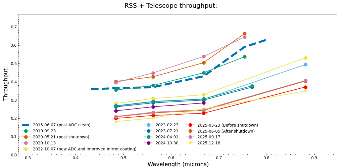
Figure 4.3: Current and historical RSS + telescope throughput values for different wavelengths (in micrometres). The most recent values are indicated with the yellow points.
