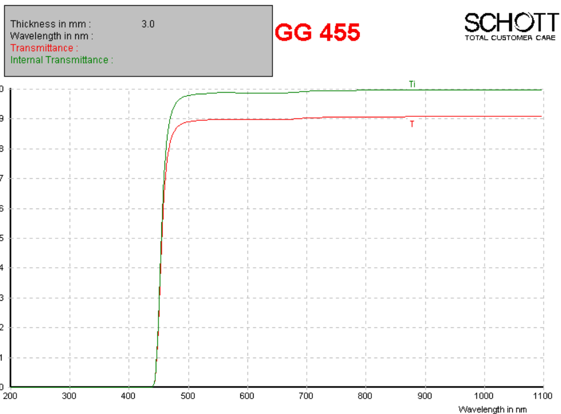
Figure A.18: Transmission curve for Blue filter PC04600.
