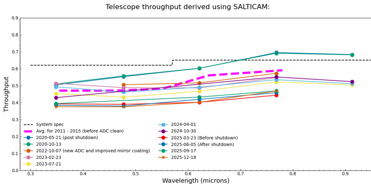
Figure 4.2: Current and historical telescope (that is, SALTICAM) throughput values for different wavelengths (in micrometres). The most recent values are indicated with the brown
