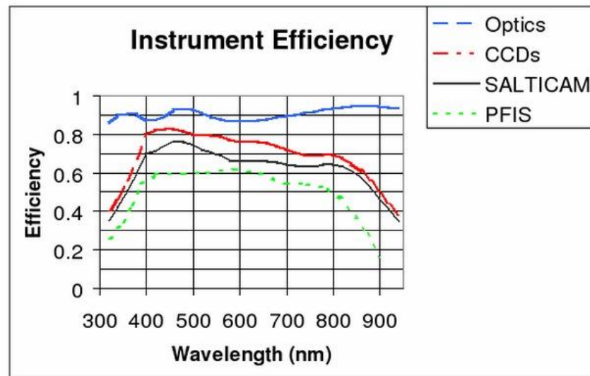
Figure 1. Instrument Efficiencies
