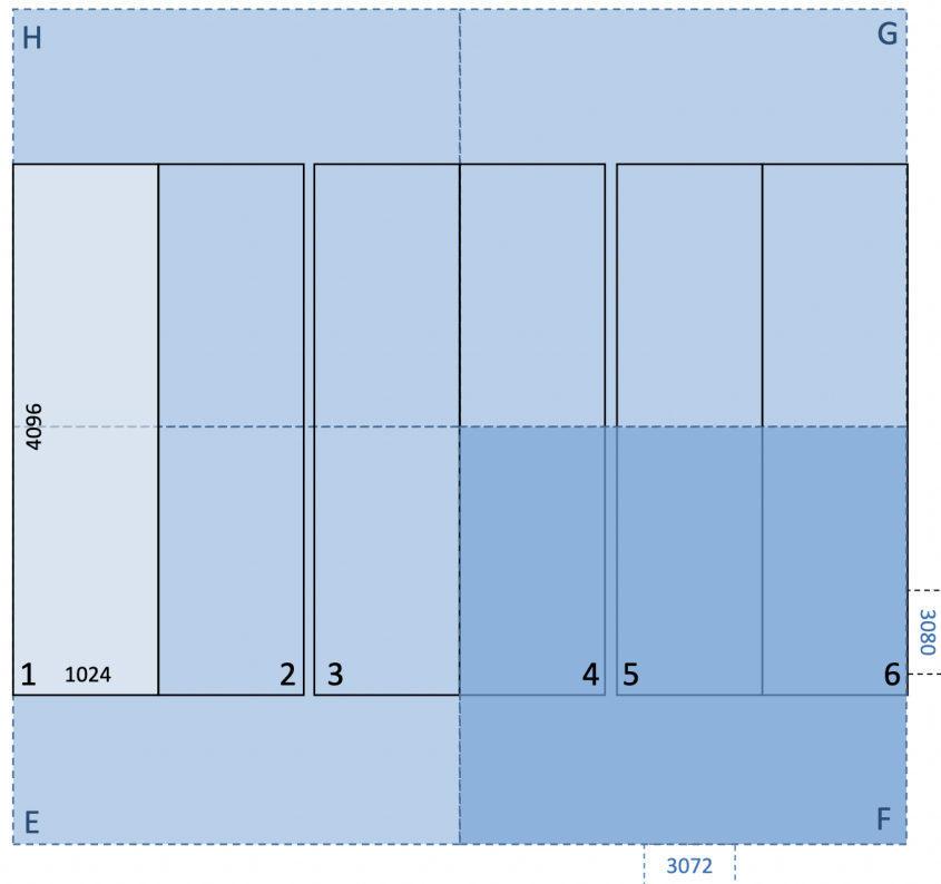
Figure A.16: New RSS detector layout with the old 3-CCD system overlaid for reference.
