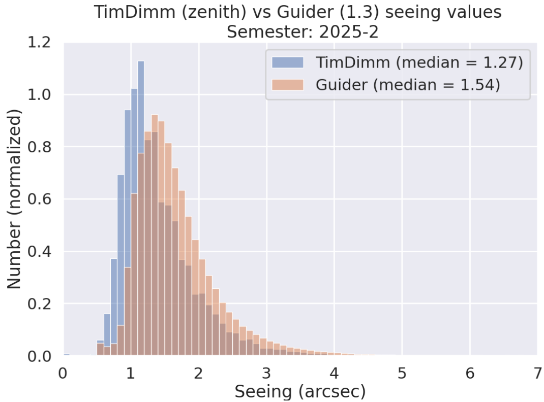
Figure 3.1: Seeing histograms from the SAAO DIMM and the SALT guider. The data are taken from the same period of time in 2025. Note that the guider data is corrected for the average airmass of SALT observations during this period. The PIs select their seeing restriction based on the intrinsic Zenith value and they now should expect a similar image quality delivered on the detector.
