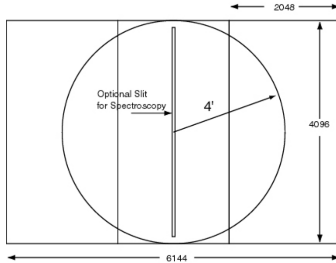
Figure 7.1: New RSS detector system with the old 3-CCD system overlaid (top). Slit position relative to the old detector for reference (bottom; old image).
